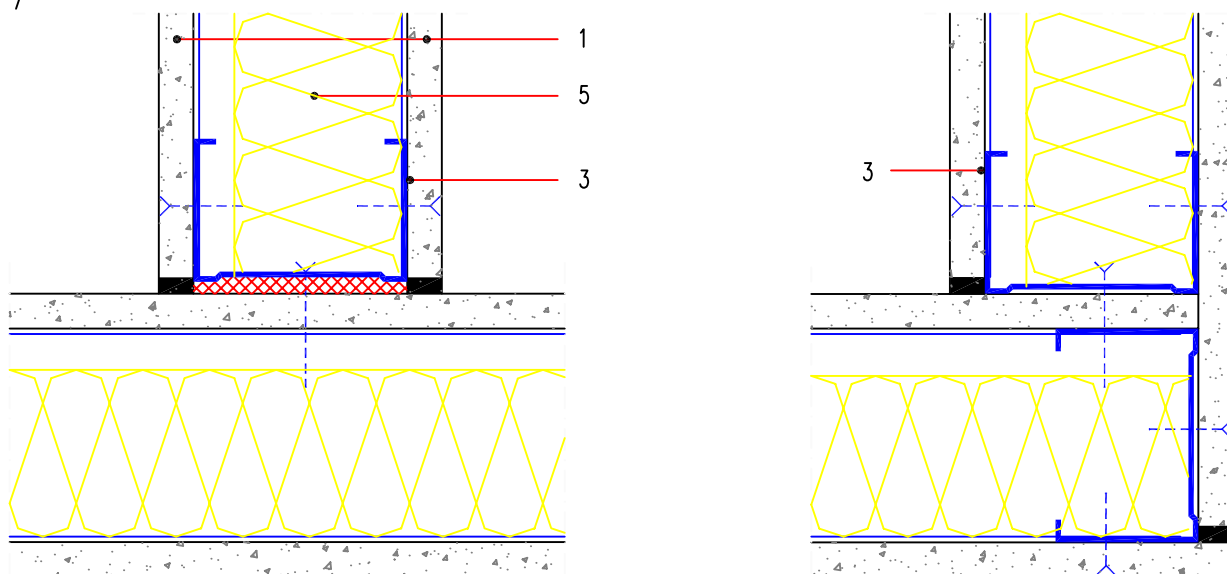
T - Junction
