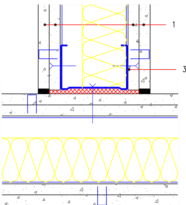
T - Junction
