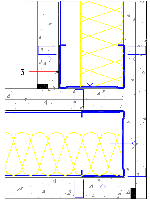
Corner Junction
