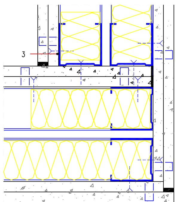
External Corner Junction
